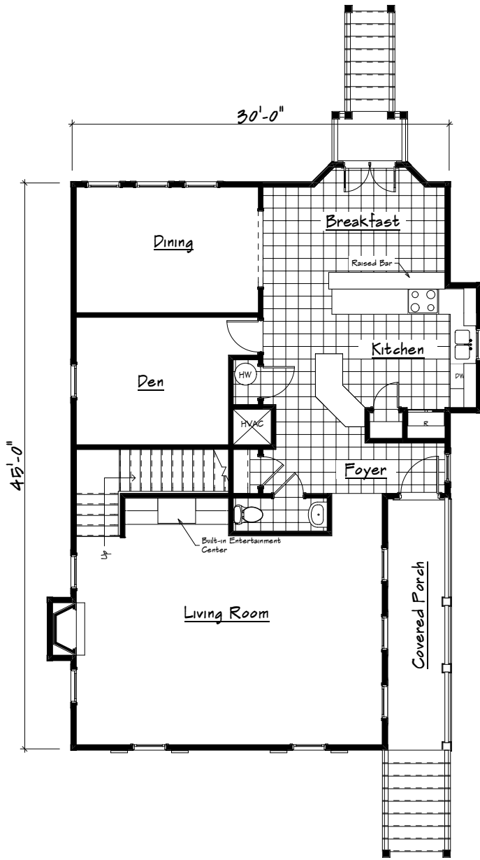
1st Floor Plan 1262 S.F.
