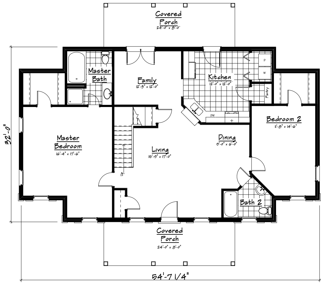
1st Floor Plan 1632 S.F.
