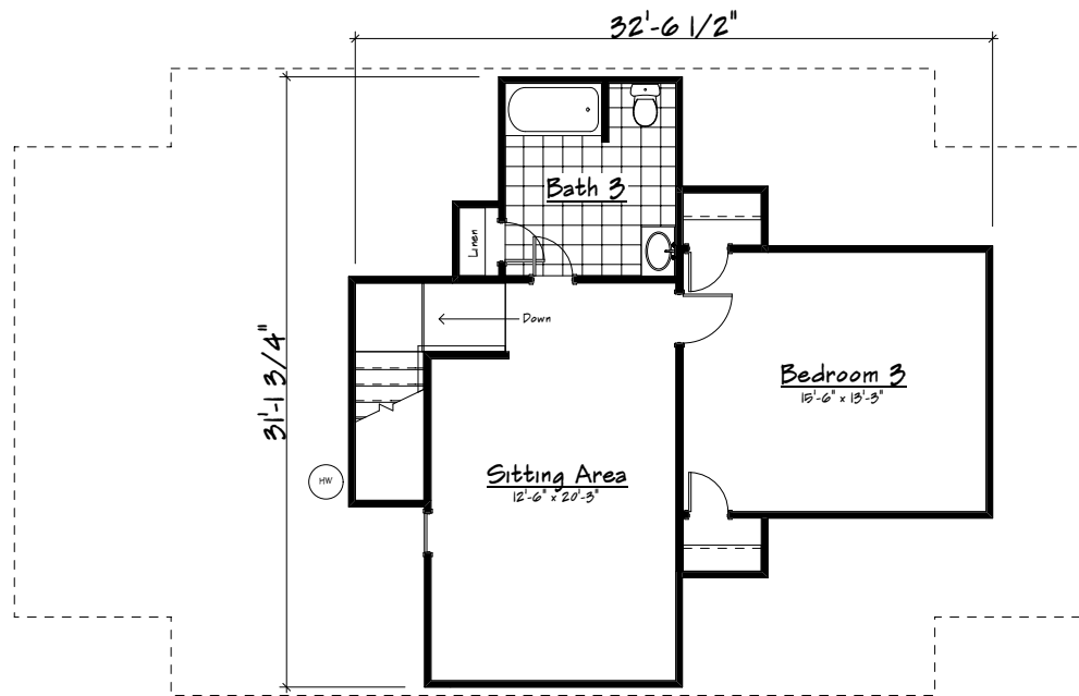
2nd Floor Plan 627 S.F.
